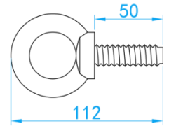
AISI316 Eyebolt
